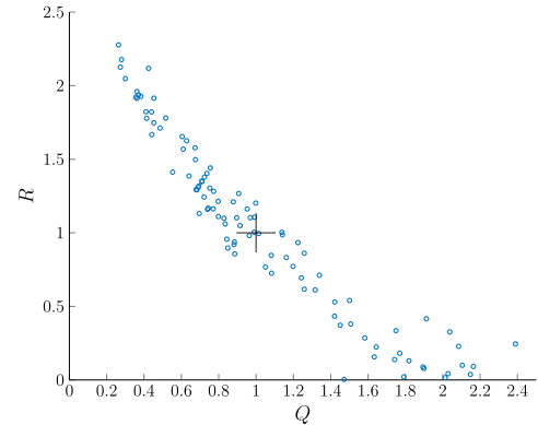
FIGURE 10. Q and R estimation for Case 4.
